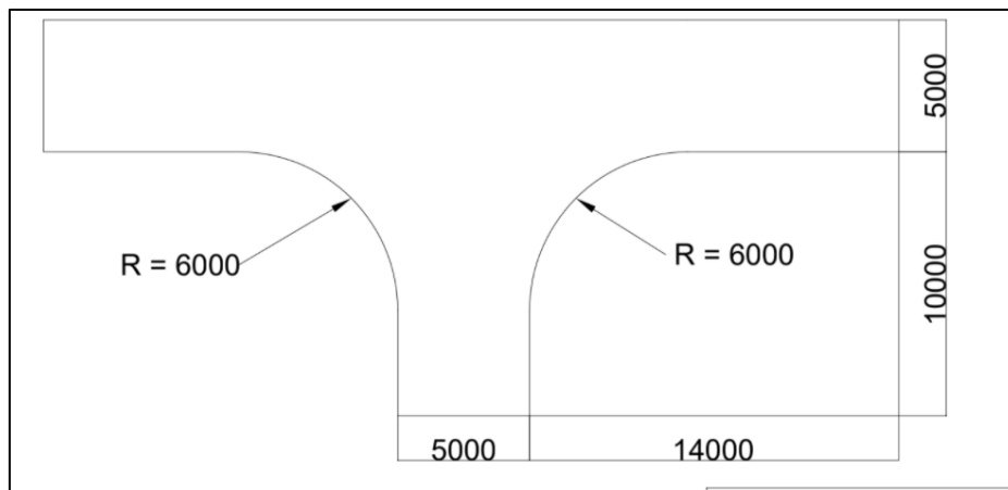
Figur 13: Vendehammer for liten lastebil (meter)
