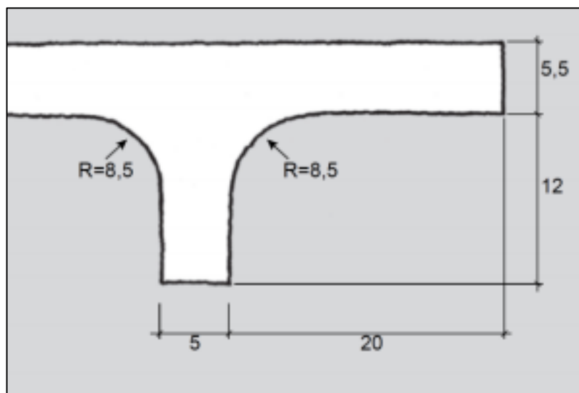
Figur 14: Vendehammer for lastebil (meter)
